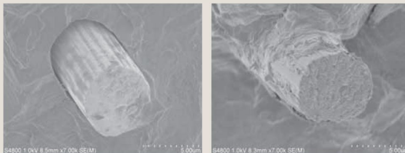
Photo 1 Interface between carbon fibers and PP resin (PP/carbon fibers = 70/30) Left: without UME X, there are gaps at the interface due to poor adhesion Right: with 1% additives of UME X, good adhesion is obtained
